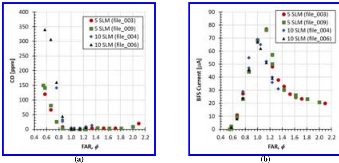
Figure 16. Carbon Monoxide "above" flame and blue flame emission intensity as a function of fuel-to-air equivalence ratio for baseline cases without plasma in CAPAC-1B: (a) Kane-May SGA91 CO measurements, and (b) 350-500 nm filtered "blue flame sensor" current measurements
